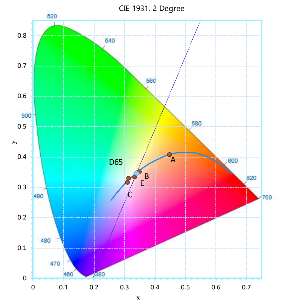
Chart 2. Chromaticity Diagram
