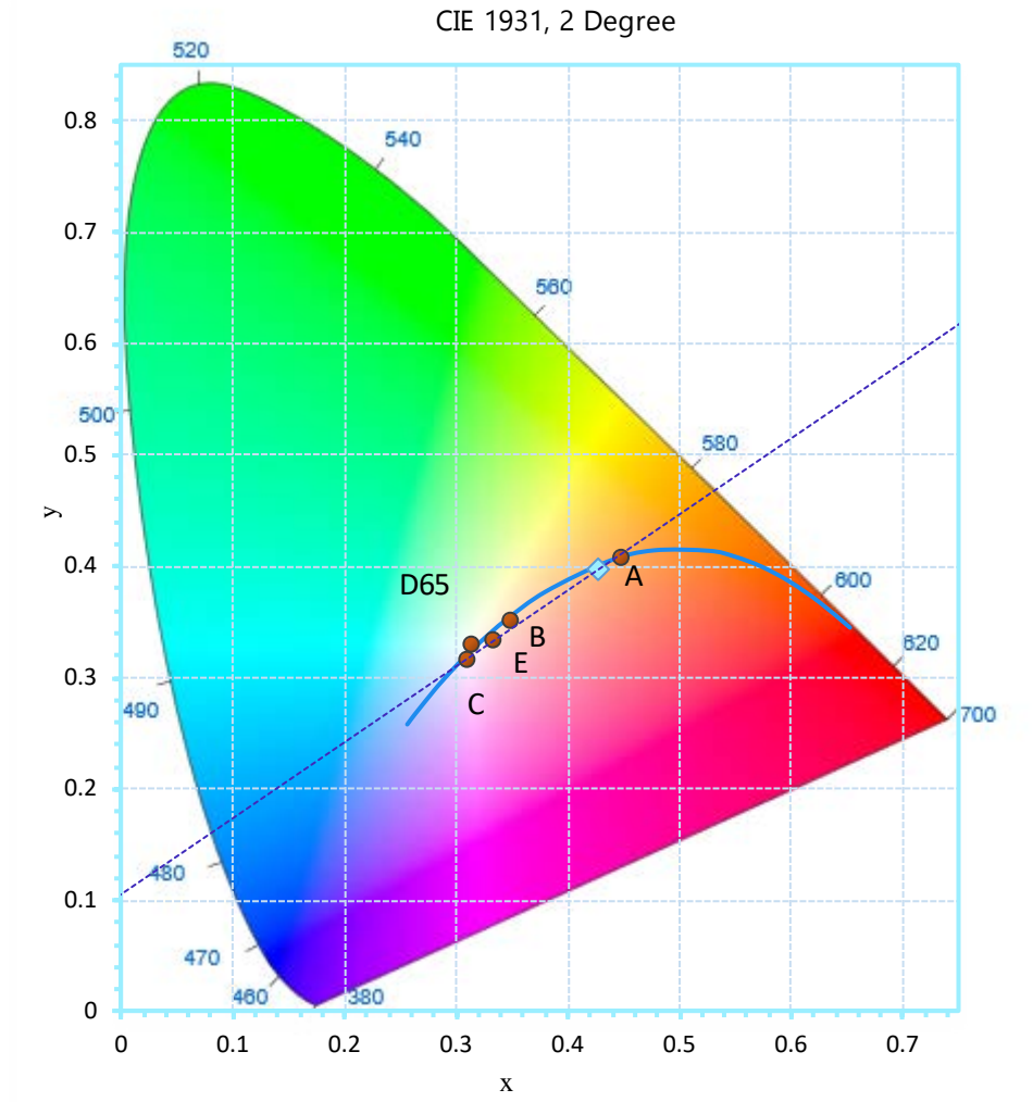
Chart 2. Chromaticity Diagram
